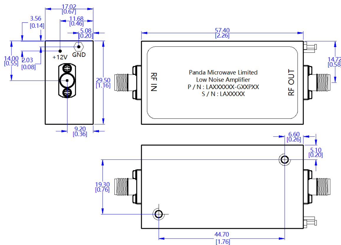
Unit: MM / [Inch], Unless otherwise specified, Outline drawing ±0.2MM ; Hole±0.1MM
